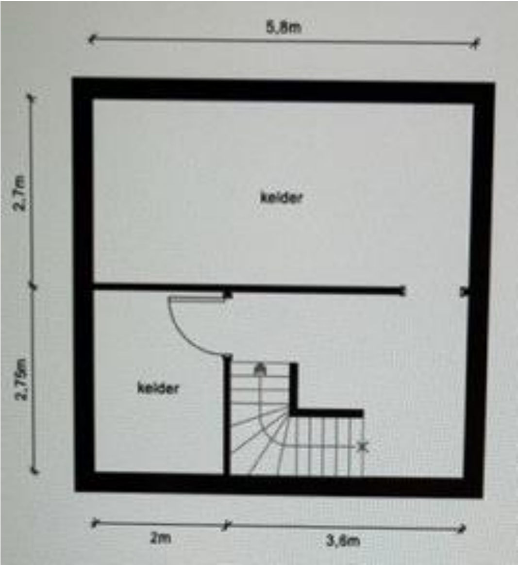
Kelderplan
